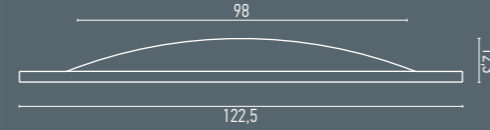
DM 501 ED: 122,5 cm ID: 98 cm D: 12,3 cm Fibre Reinforced Plastic (FRP)
