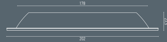
DM 512 ED: 202 cm ID: 178 cm D: 23,5 cm Fibre Reinforced Plastic (FRP)
